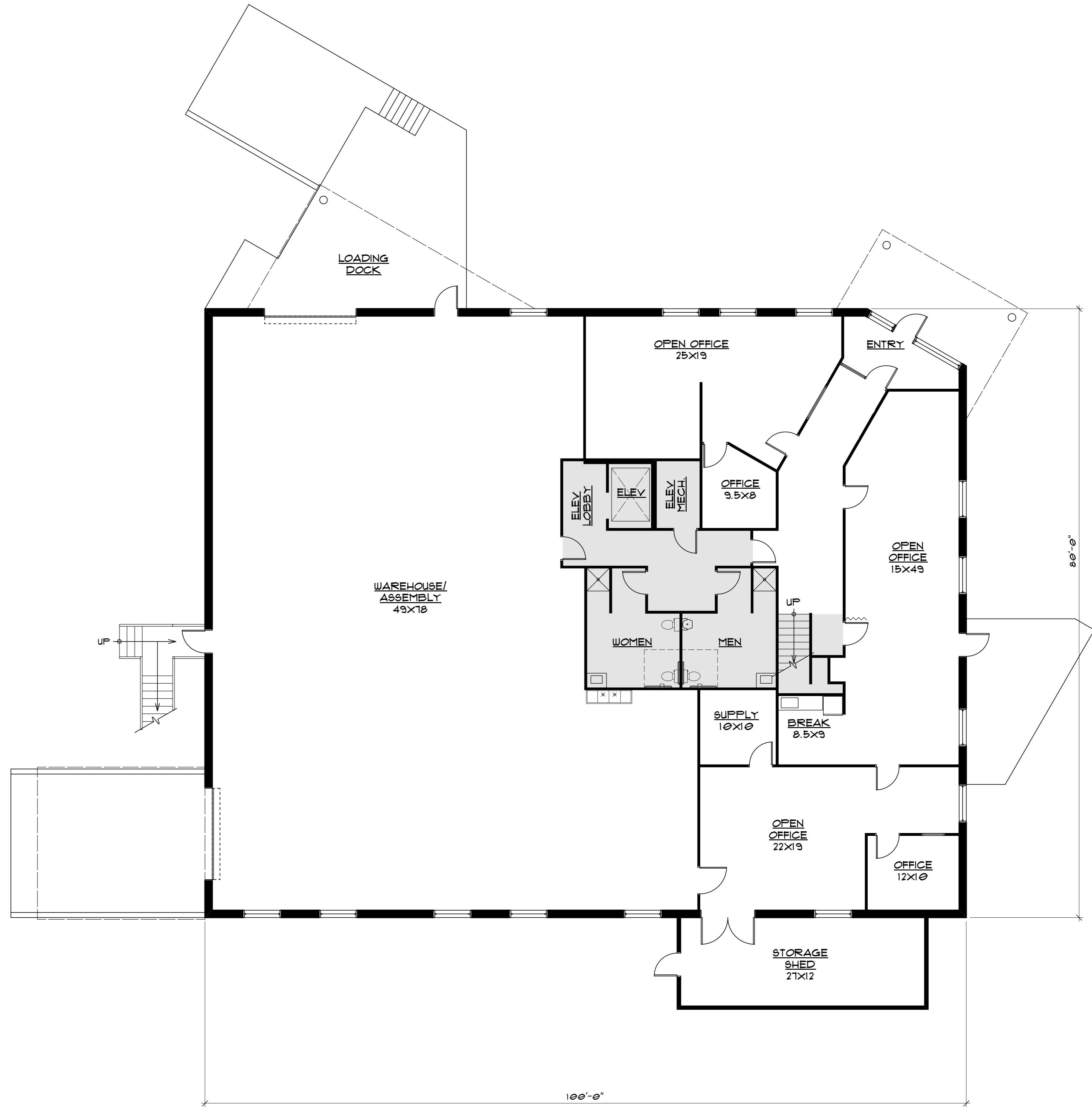
PACIFIC DRIVE BUILDING - FIRST FLOOR PLAN 1/8" = 1'-0"
