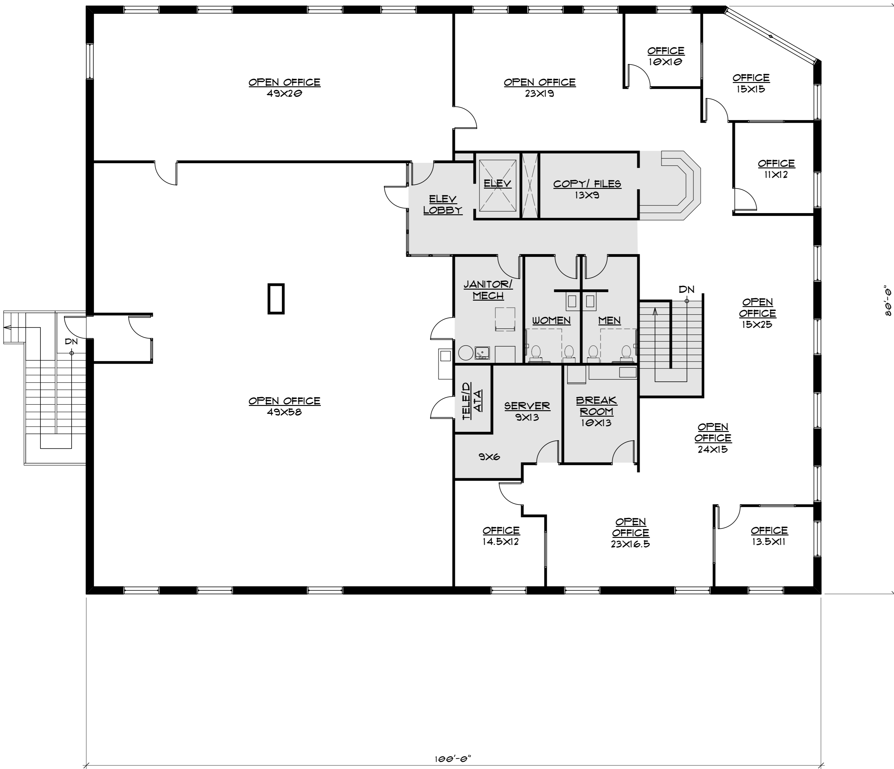
PACIFIC DRIVE BUILDING - SECOND FLOOR PLAN 1/8" = 1'-0"
